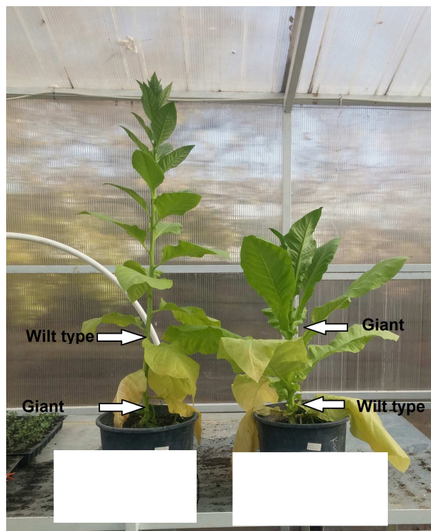
Figure 1. Reciprocal grafting at Nicotiana in this study.
